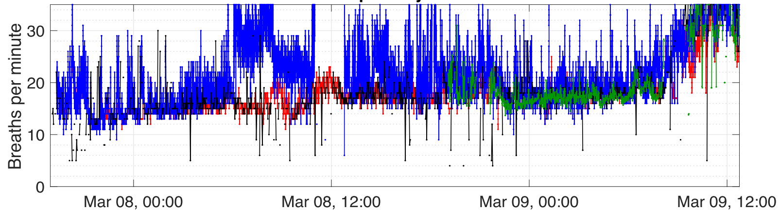
Respiratory rate
